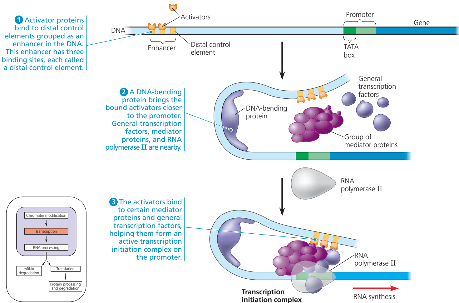
▲ Figure 18.10 A model for the action of enhancers and transcription activators.
